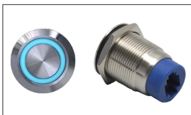
Model 013-100 Easy Plug Push-Button with RJ9 connector for easy installation and long term reliability.
