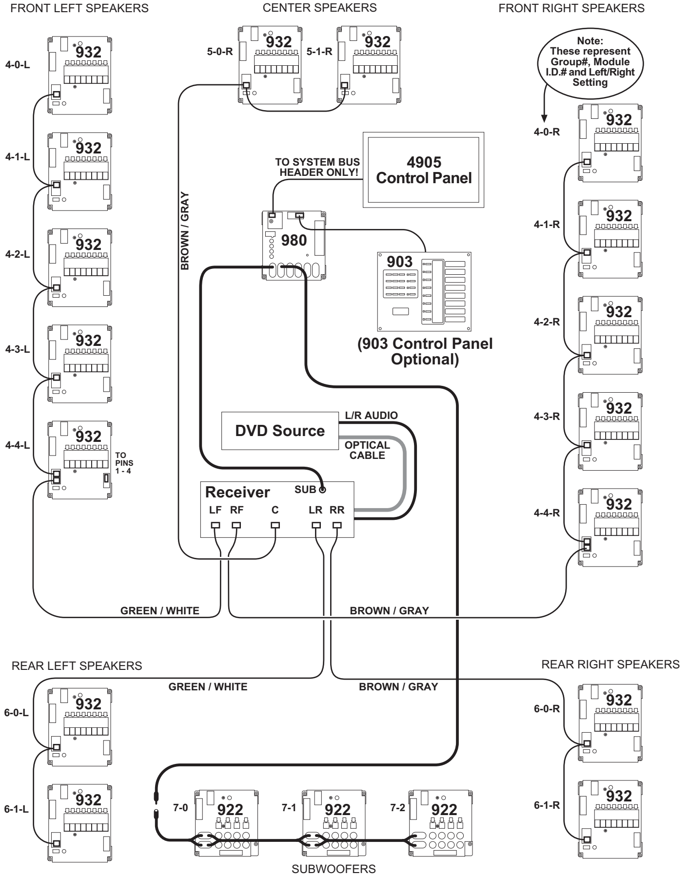
Figure 2. Wiring diagram (System Bus not shown).
