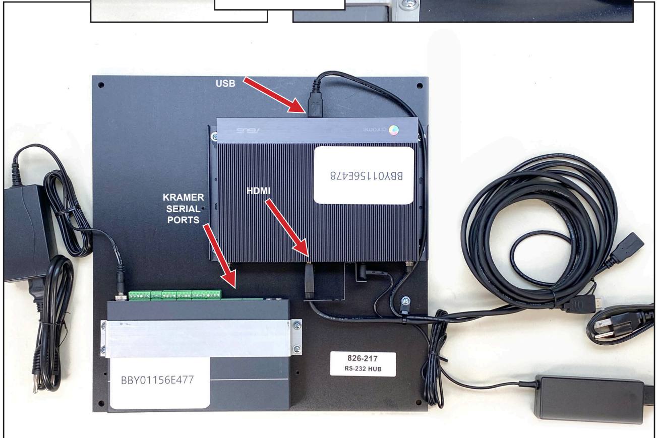
CHROMEBOX CONNECTIONS TO CABINET 1, TOUCHSCREEN.
