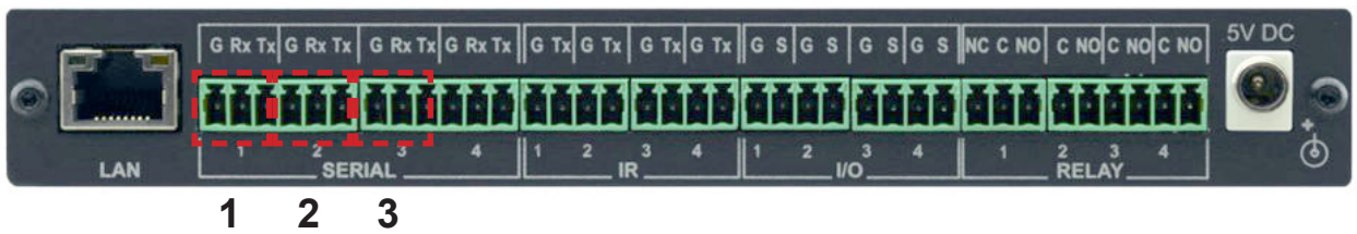
KRAMER SL240C SERIAL PORTS PORT 1: FROM 0970A-1, CABINET 3, 826-216 PORT 2 FROM MH2-HS, CABINET 3, 826-216 PORT 3 FROM 826-220A
