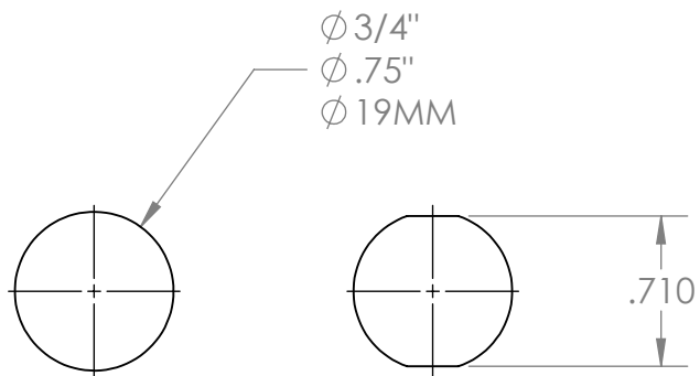
PANEL CUTOUT
