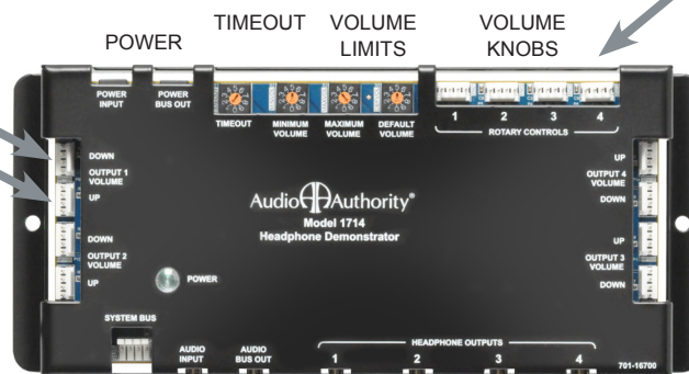
AUDIO BUS
