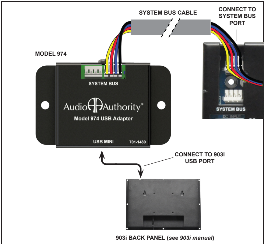
974 connection diagram.
